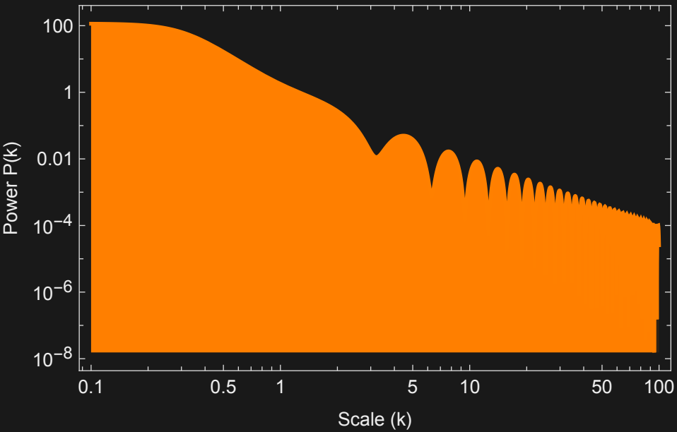
CMB Power Spectrum: The 1/k^4 Noise Floor ( R=1.15428 )
